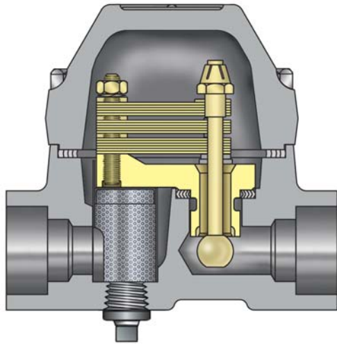
The Velan Steam Trap
